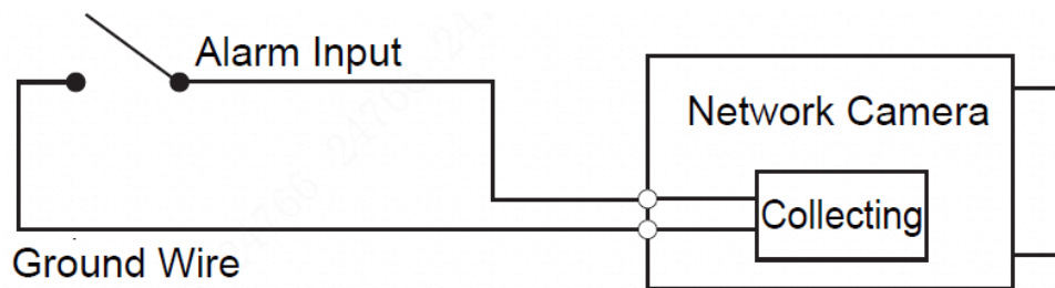
Figure 1-3 Alarm input
